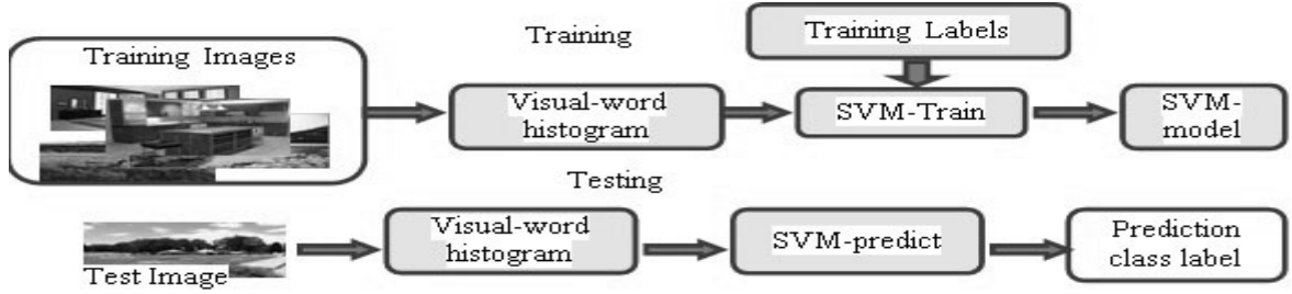
Figure 4: Learning Based Object Detection Processes
