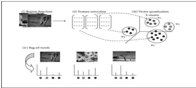
Figure 1: BoVW Construction Steps
