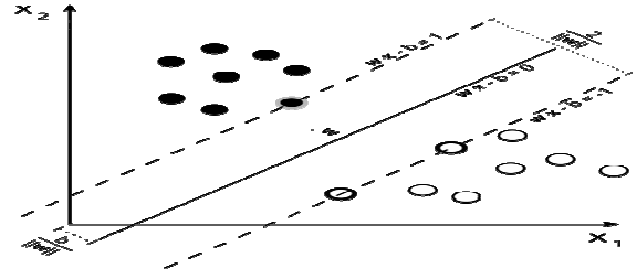
Figure 3: An Example of Binary SVM Classification, Separating Two Classes (Black Dots from White Dots)
