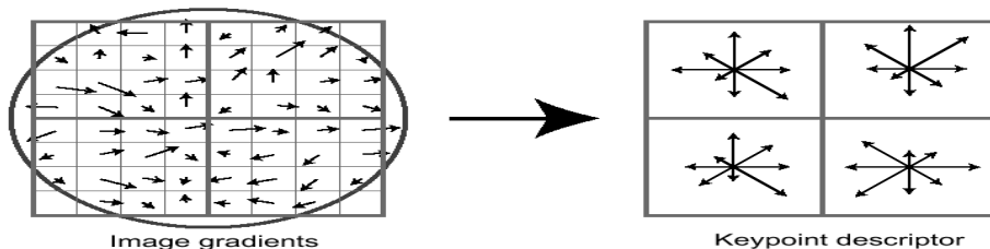
Figure 2: SIFT Descriptor
